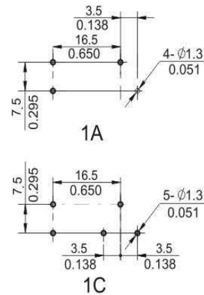
安装尺寸图 (底视图) Mounting (Bottom view)
